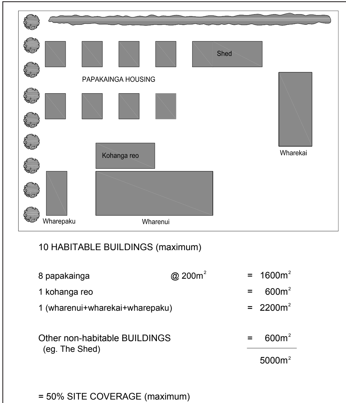
Diagram 15.1 Provision for PAPAKAINGA HOUSING (an example)
