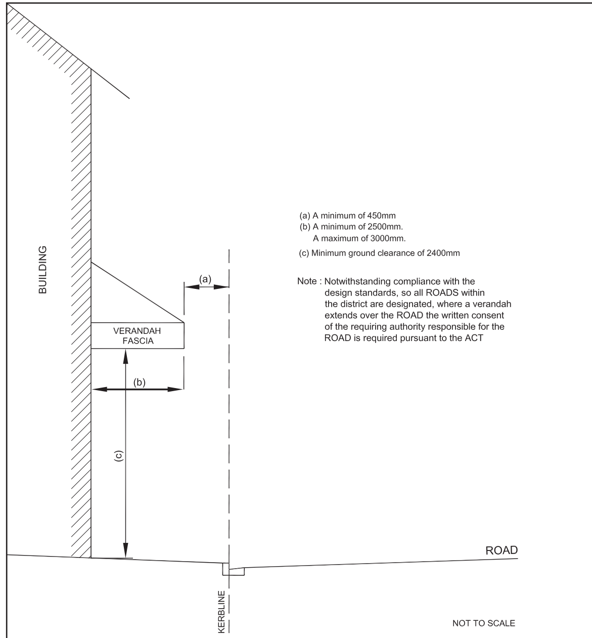
Diagram 25.1 Verandah design standards within the DEFINED RETAIL FRONTAGE
